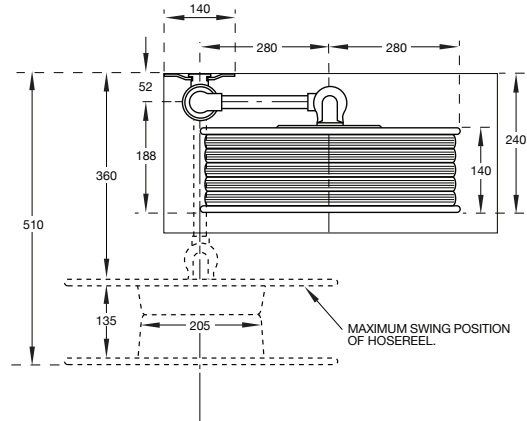
BACK MOUNTING
