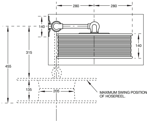
SIDE MOUNTING
